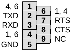
Figure 4: COM Connector
